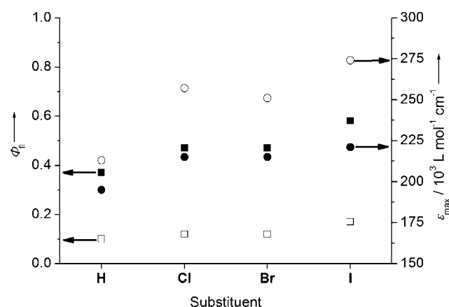
Figure 2. Influence of halogen atoms on the optical properties (squares: \Phi_{\text{em}} ; circles: \epsilon_{\text{max}} ) of squaraines 5a–d (filled symbols) and 6a–d (open symbols).
